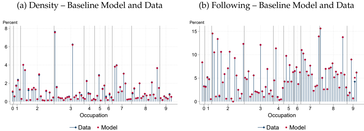
Figure 8: Model Fit
