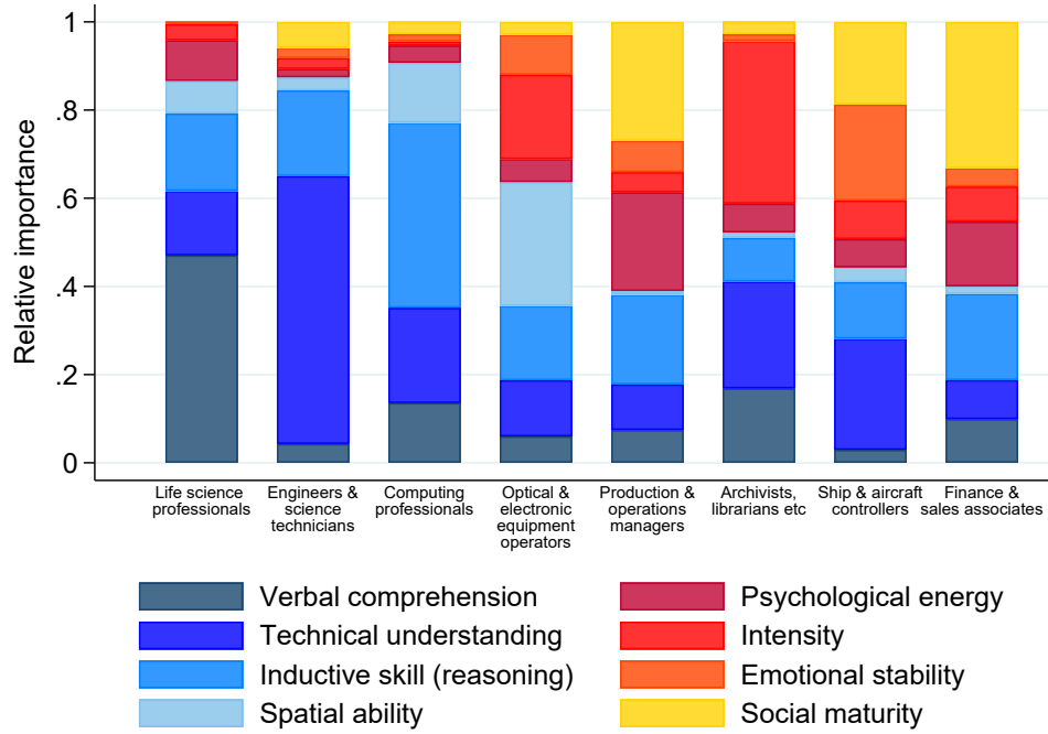
Figure 7: Factor Importance
