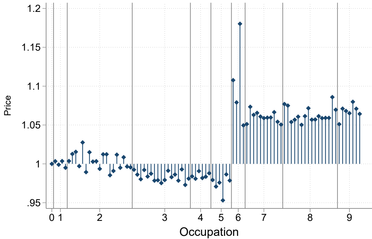
Figure A.20: Price changes in General Equilibrium
